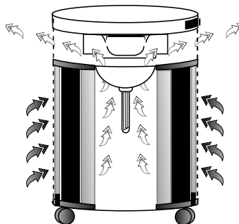
The TitanClean reflector positioned in the center of the filter chamber
